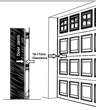
EMB-A-SEAL FOR SECTIONAL DOOR
