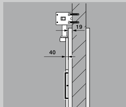
Max. door overlap 40 mm
