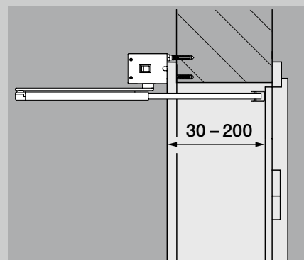
Reveal depth 30 - 200 mm
