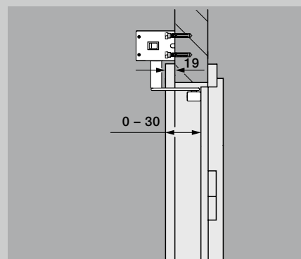
Reveal depth 0 - 30 mm
