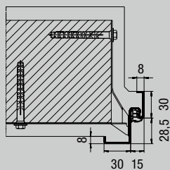
Profile 11100
