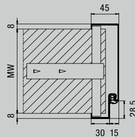
Profile 21101
