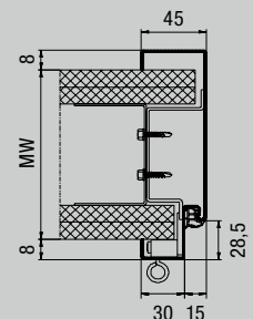
Profile 21120
