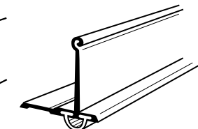
Aluminium bottom rail (extrusion)
